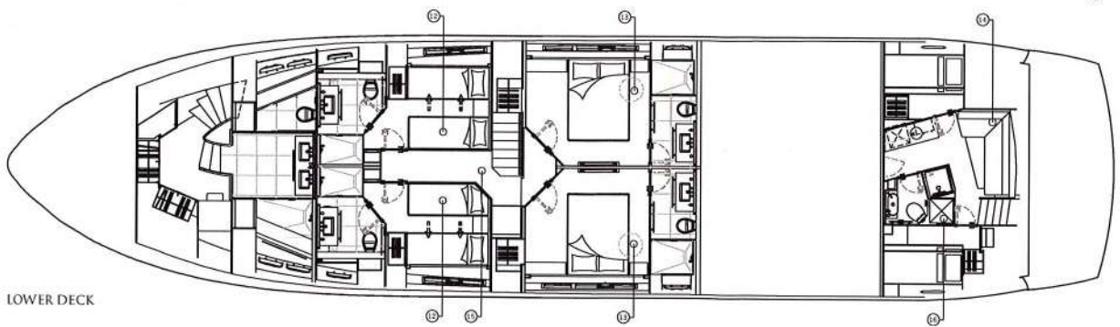
MAIN DECK
