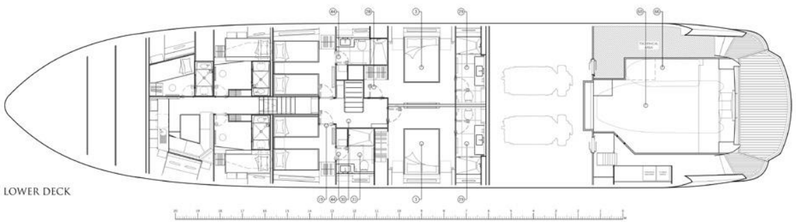
MAIN DECK
