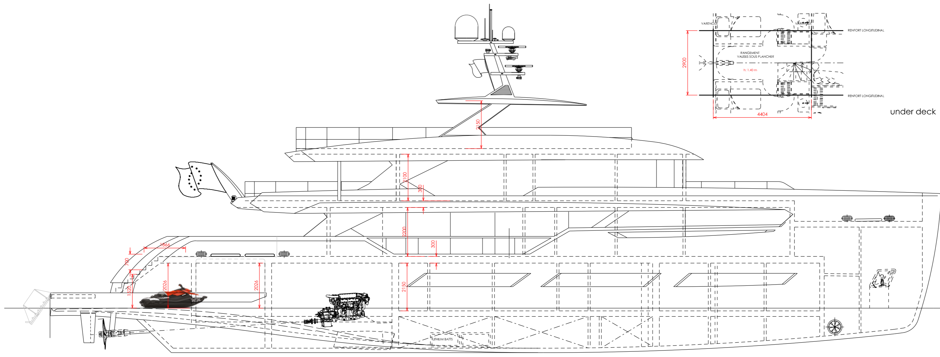
lower deck
