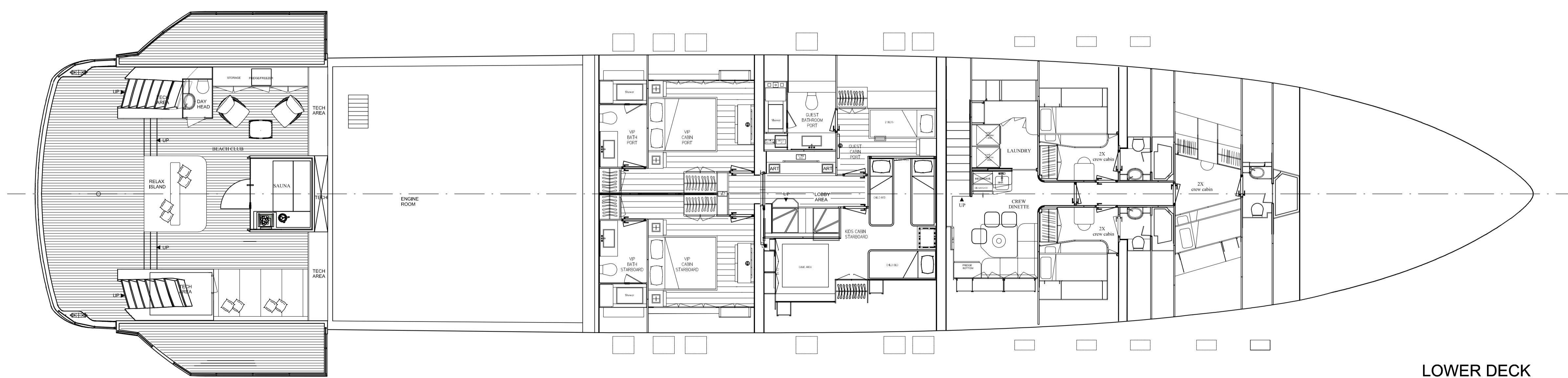
LOWER DECK
