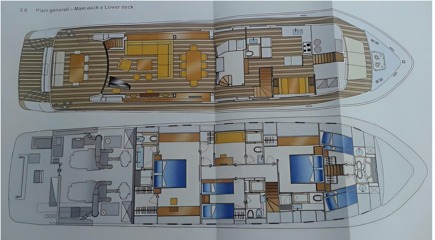
2010 Sanlorenzo SL88 Exact Layout – GA
