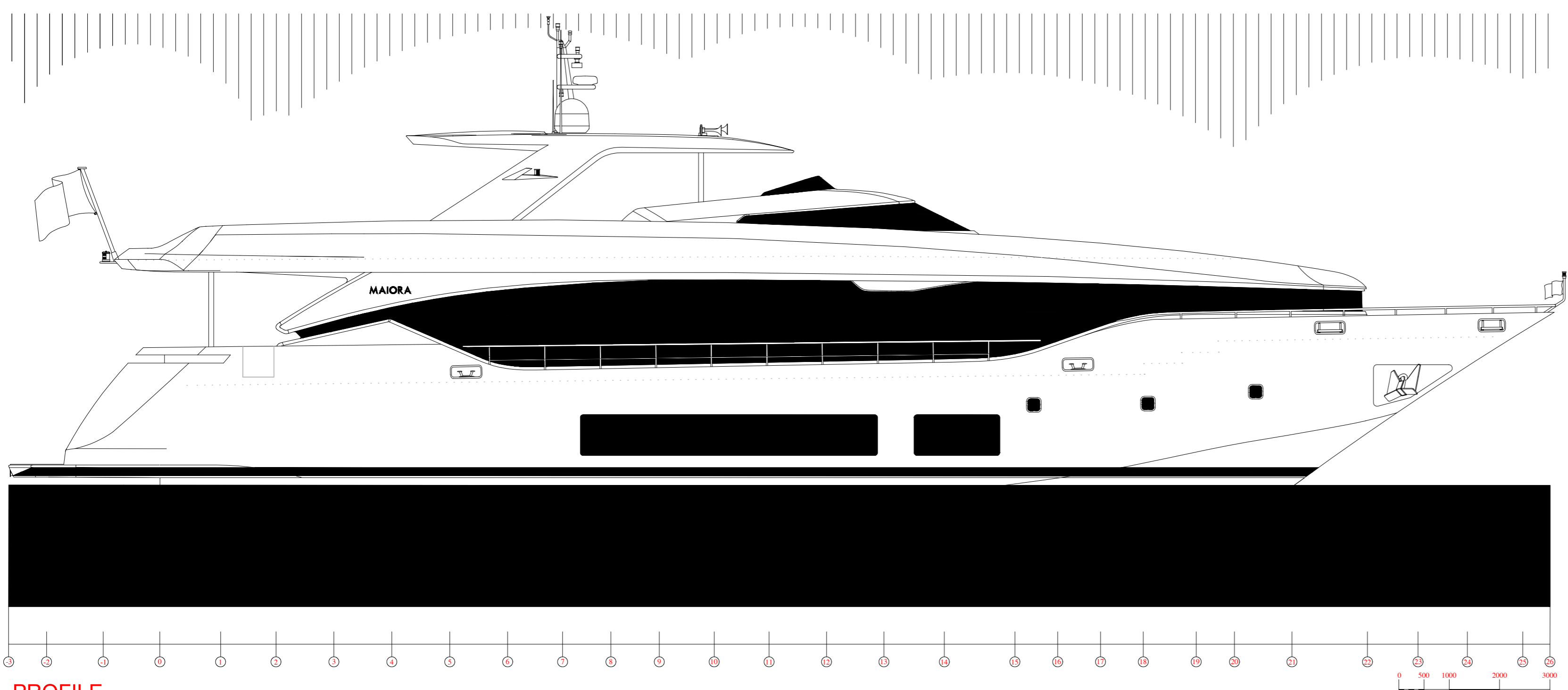
PROFILE SCALA METRICA
