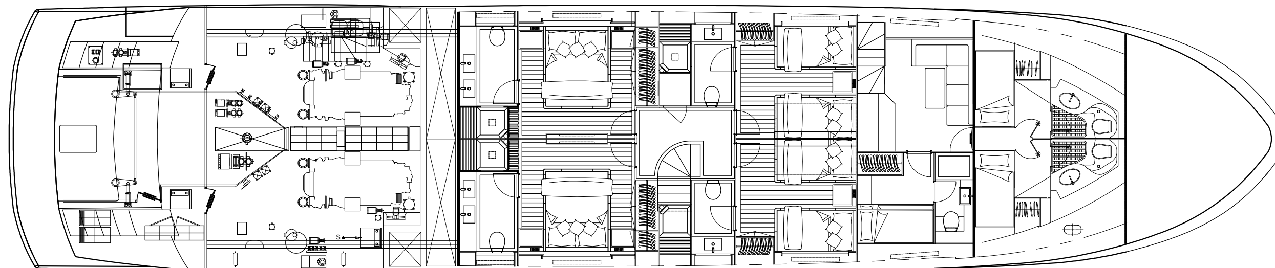
LOWER DECK 24_2_15
